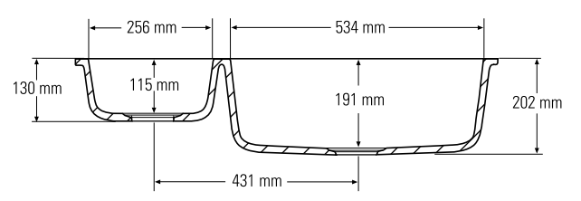
Front cross-section
