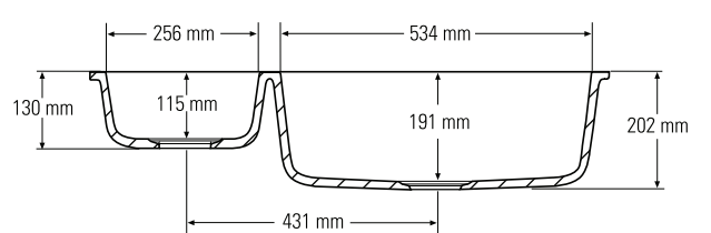
Front cross-section
