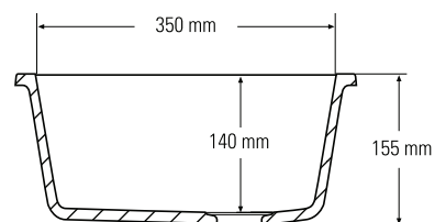
Side cross-section
